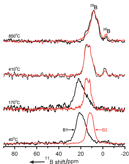
Figure 2. 11 B spin-echo MAS NMR spectra of SiO 2 NPs treated with B1 (black) and B2 (red). Samples were annealed in air at the specified temperatures. Trigonal ( 3 B) and tetrahedral ( 4 B) boron species are indicated.
